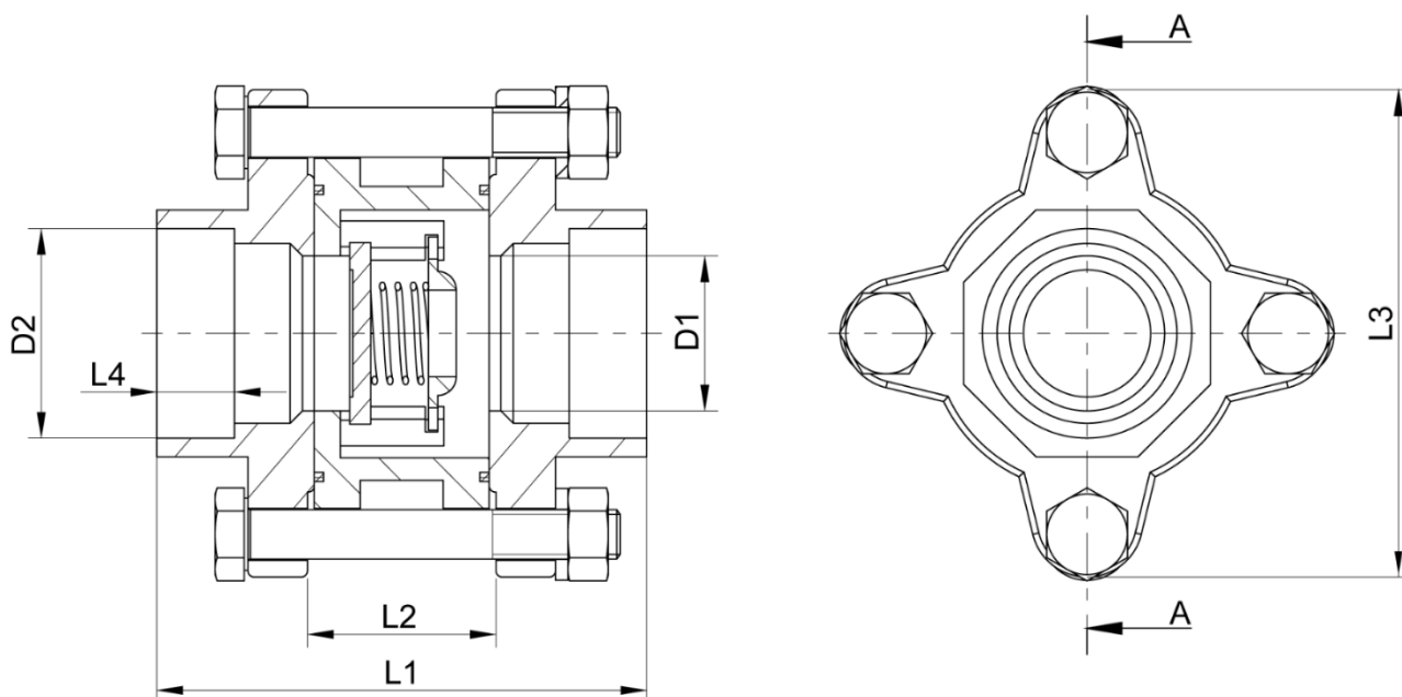
A-A cross section
