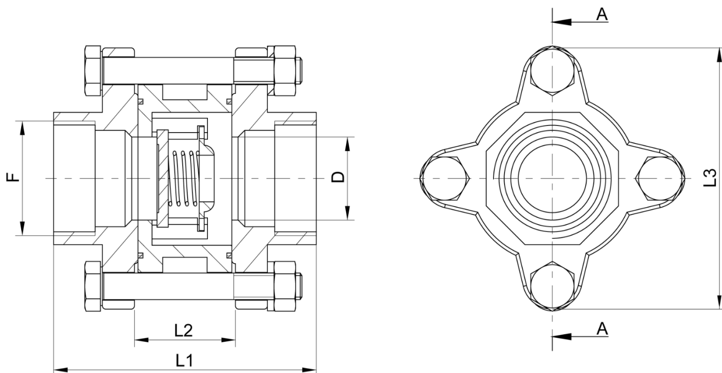
A-A cross section
