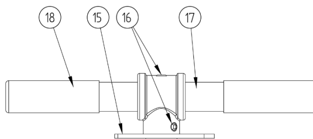
Handle DN 65 - 150 (2"1/2 - 6")
